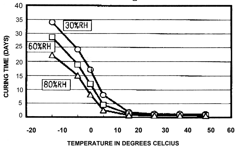
P-201 Curing Time
